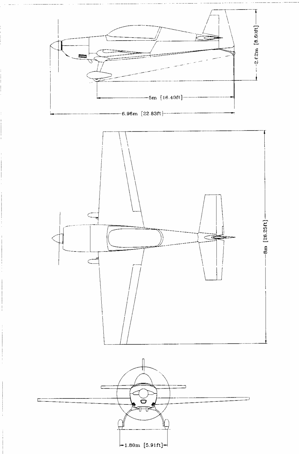
Three-View EXTRA 300L Figure 2
